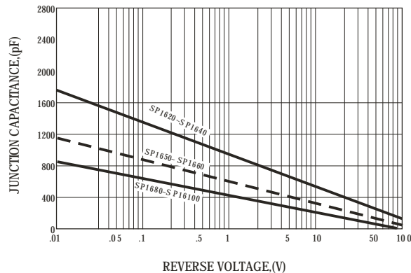
FIG.4-TYPICAL JUNCTION CAPACITANCE
