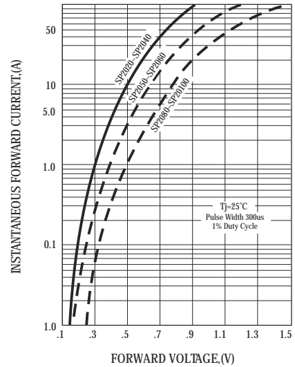
FIG.2-TYPICAL FORWARD CHARACTERISTICS
