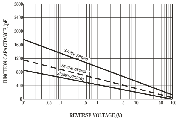
FIG.4-TYPICAL JUNCTION CAPACITANCE
