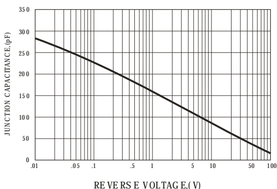
FIG. 4-TYPICAL JUNCTION CAPACITANCE
