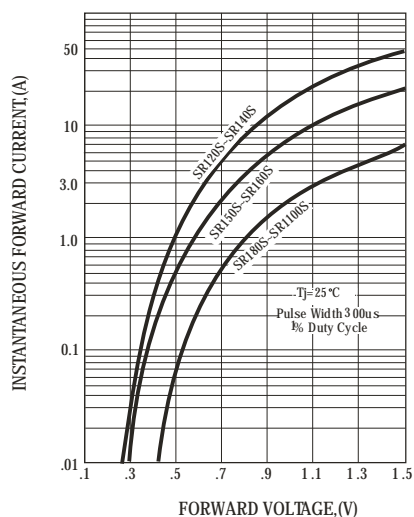
FIG.2-TYPICAL FORWARD CHARACTERISTICS
