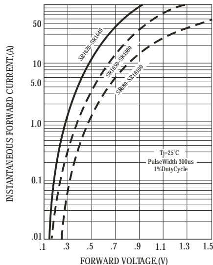
FIG.2-TYPICAL FORWARD CHARACTERISTICS
